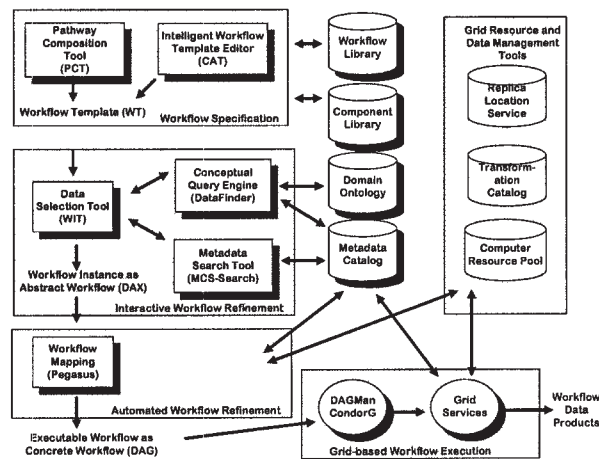
Figure 1: The SCEC/CME system supports workflow specification, refinement, and grid-based execution.
